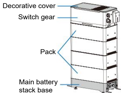
Main battery stack
