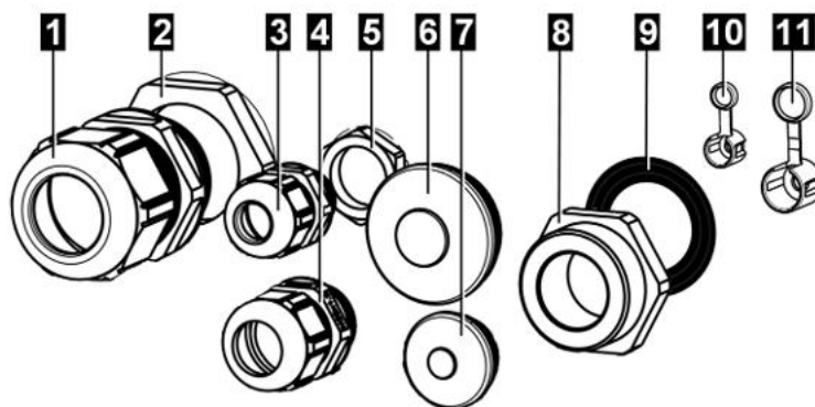
Abb. 3-2: Montagematerial
