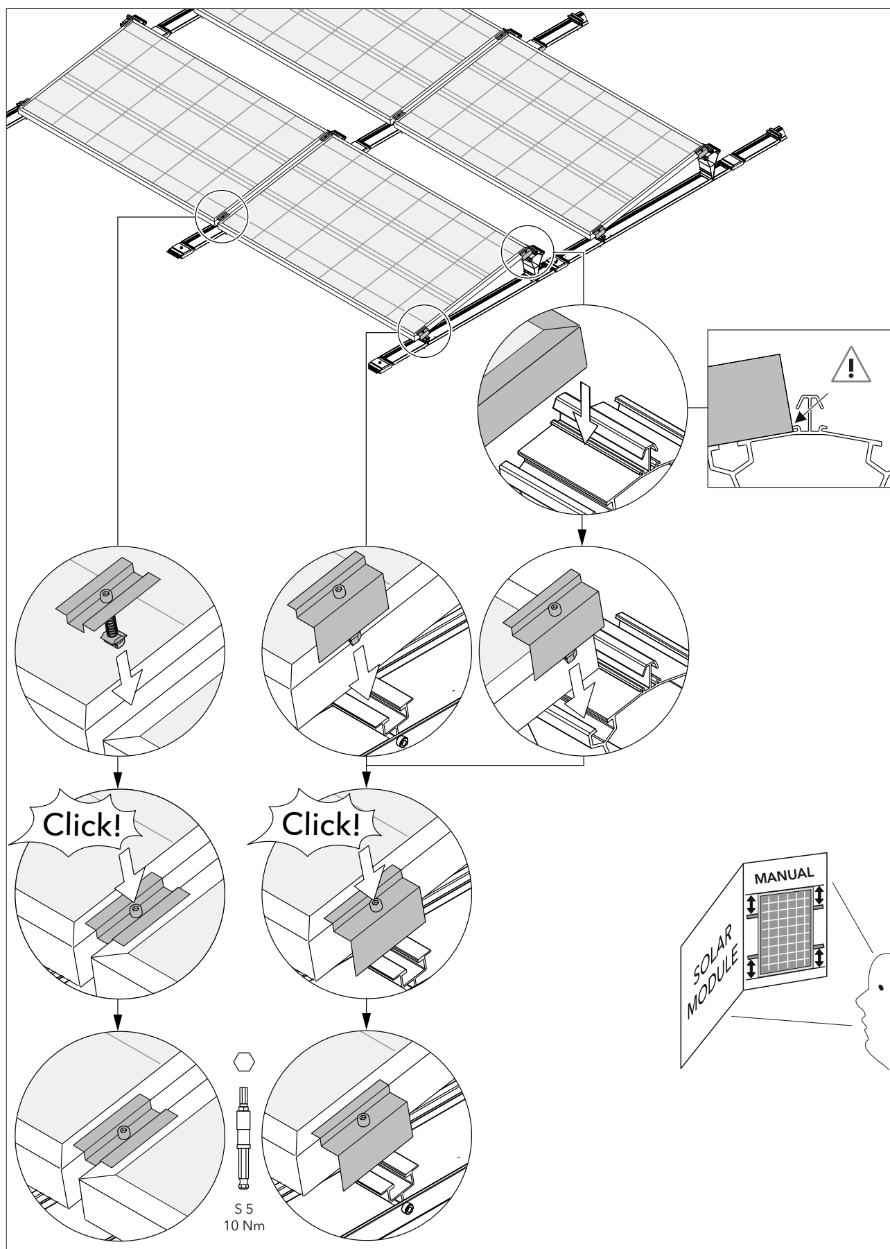
TRIC F duo 10° Süd / South / Sud / Zuid
