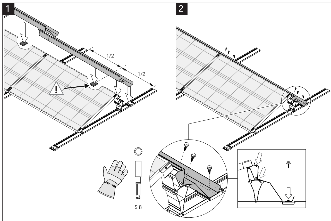
TRIC F duo 17/18° Süd / South / Sud / Zuid
