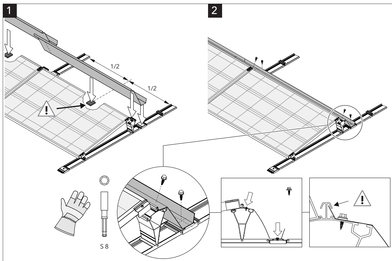
TRIC F duo 10° Süd / South / Sud / Zuid
